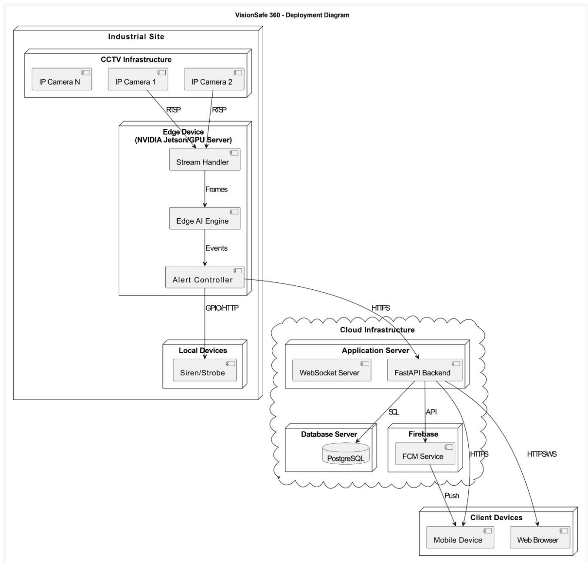
Figure [15] – Deployment Diagram
