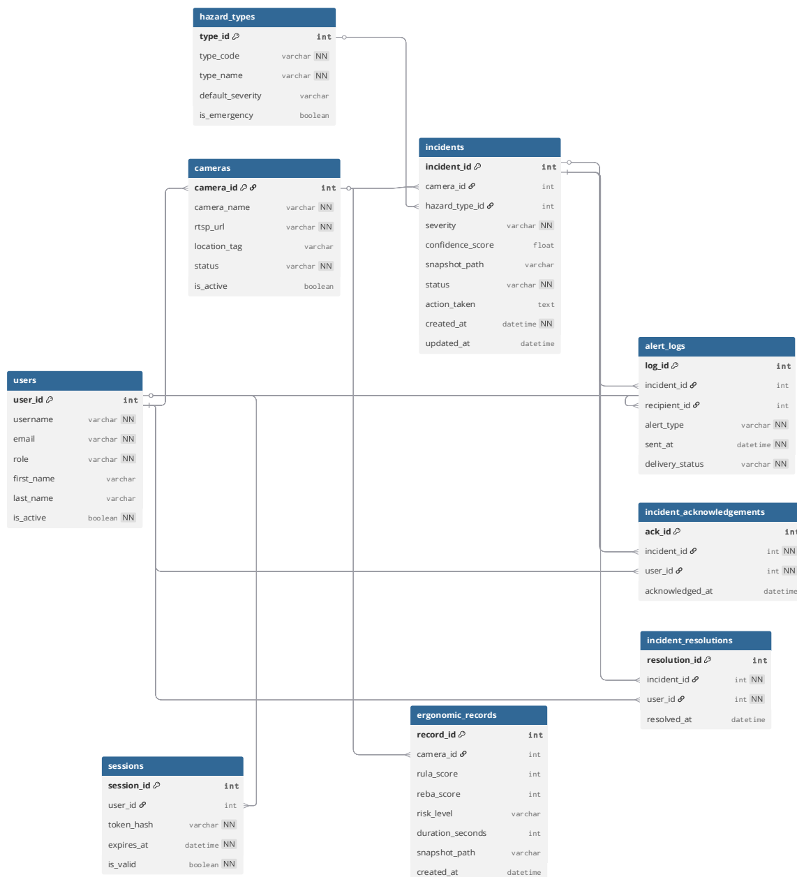
Figure [19]: Entity-Relationship Diagram (ERD)
