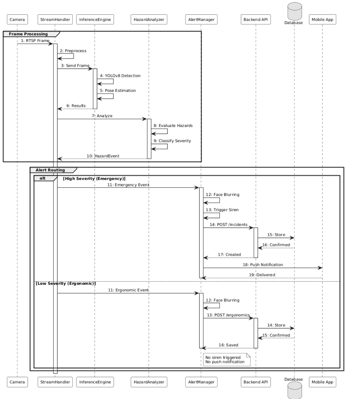
Figure 3-8: Hazard Detection Sequence Diagram
