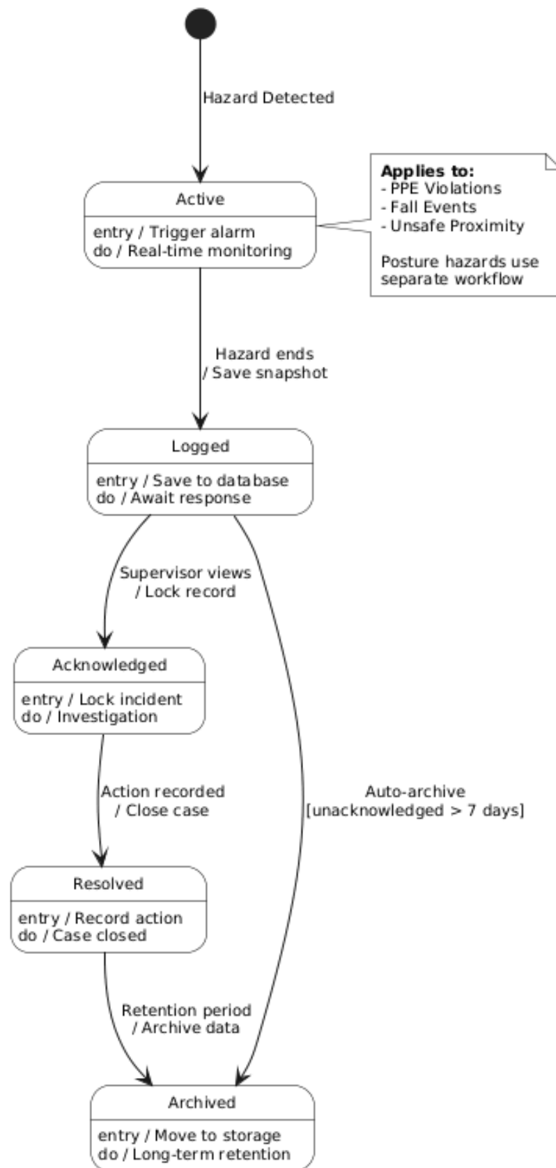
Figure [13] – State Diagram
