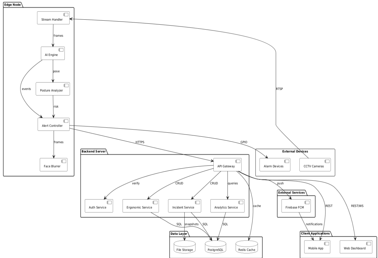
Figure [14] – Component Diagram
